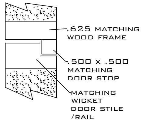
WICKET DOOR / FRAME DETAIL "B"
